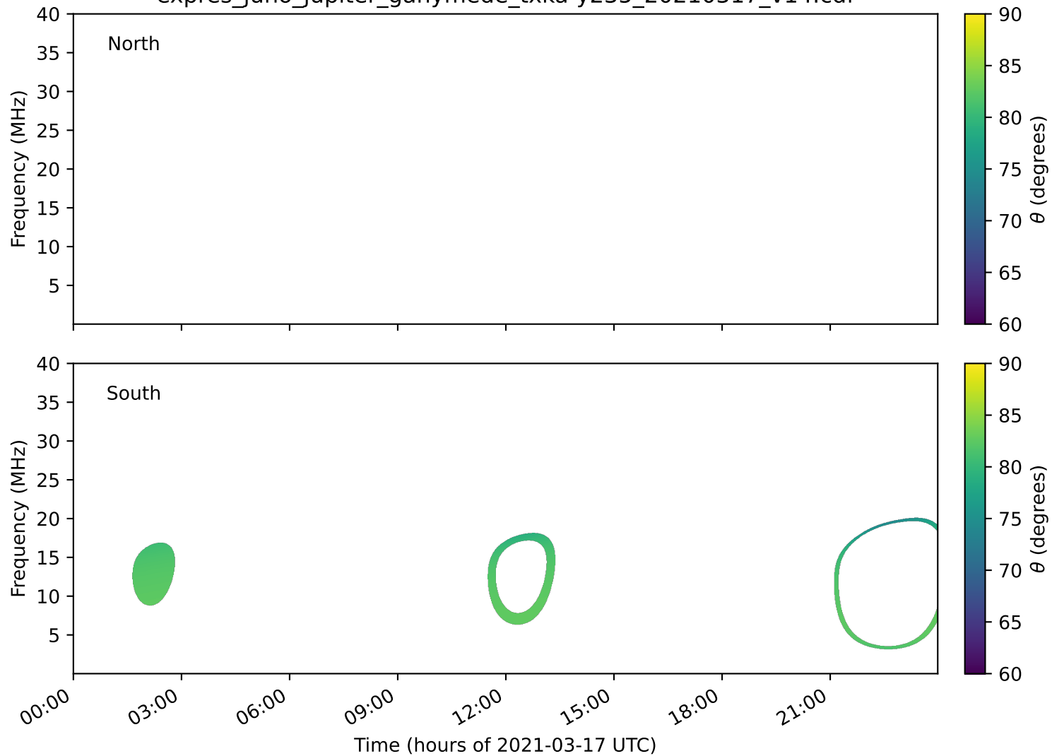
expres_juno_jupiter_ganymede_txka-y235_20210317_v14.cdf
