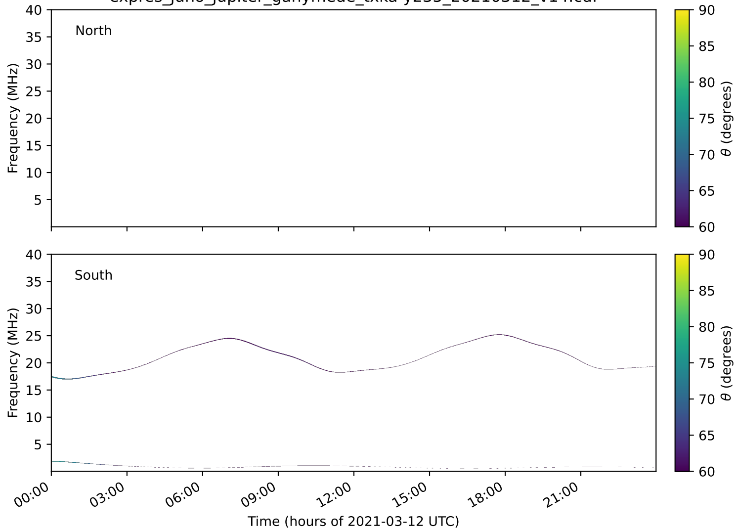
expres_juno_jupiter_ganymede_txka-y235_20210312_v14.cdf
