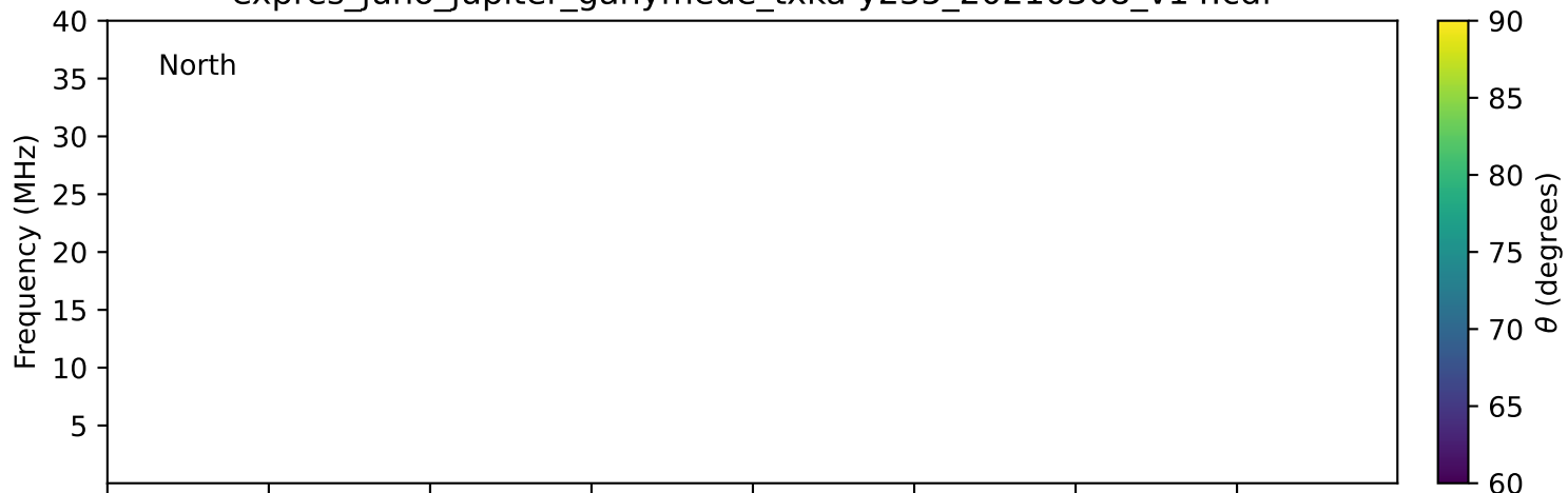
expres_juno_jupiter_ganymede_txka-y235_20210308_v14.cdf
