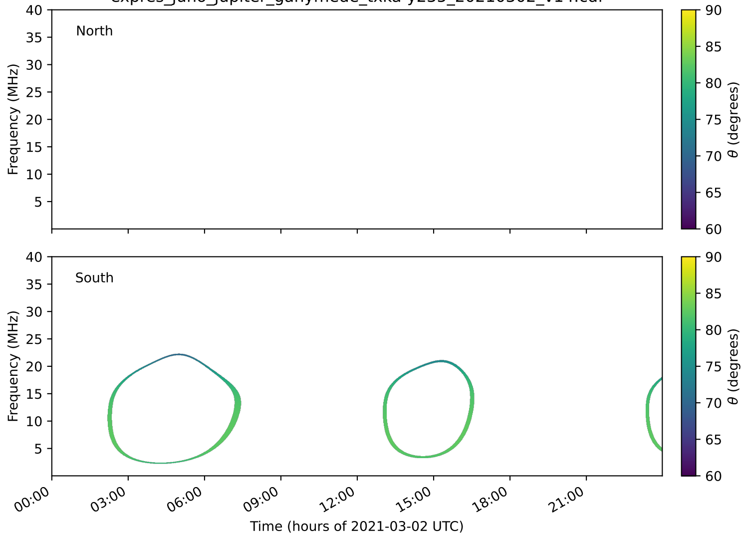
expres_juno_jupiter_ganymede_txka-y235_20210302_v14.cdf
