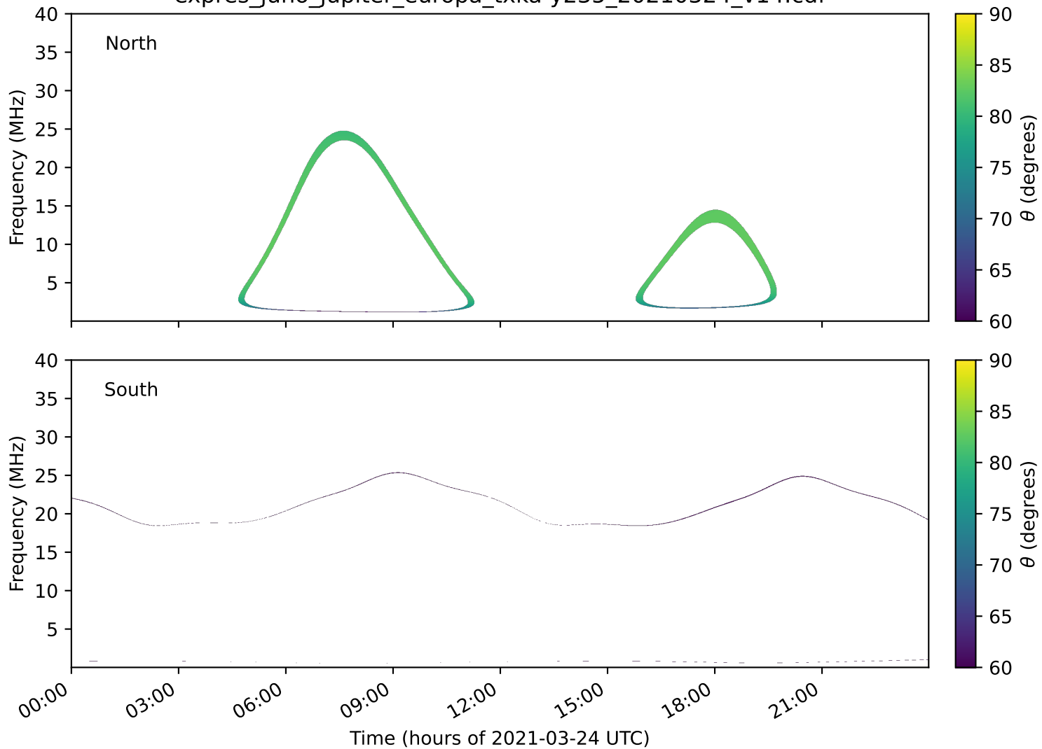
expres_juno_jupiter_europa_txka-y235_20210324_v14.cdf
