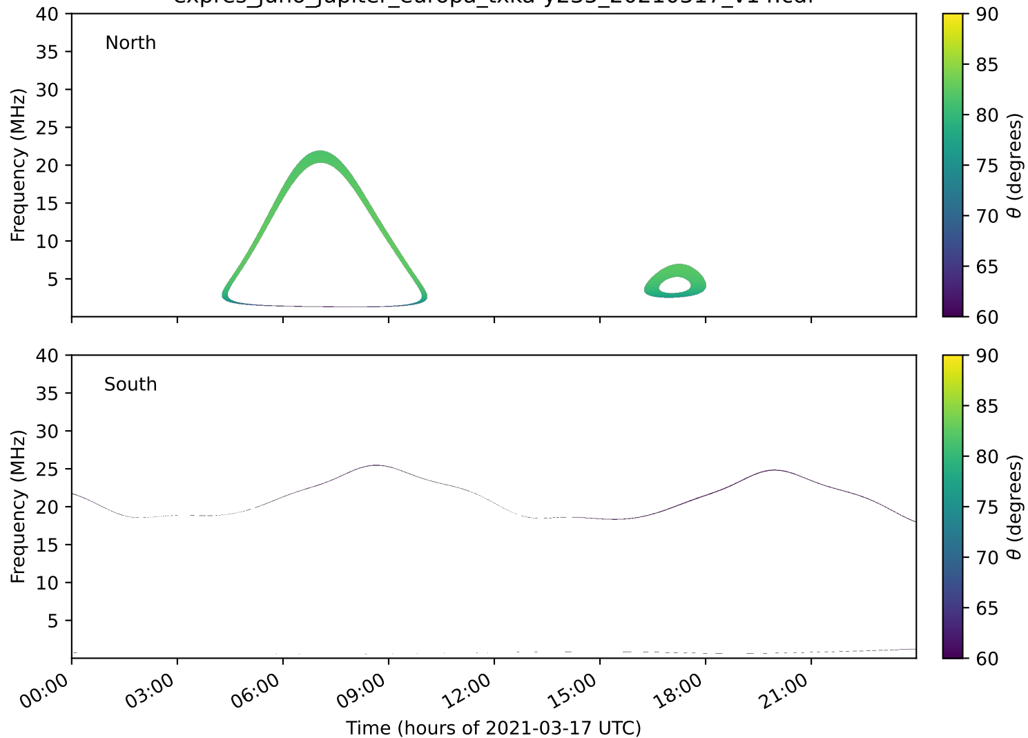
expres_juno_jupiter_europa_txka-y235_20210317_v14.cdf
