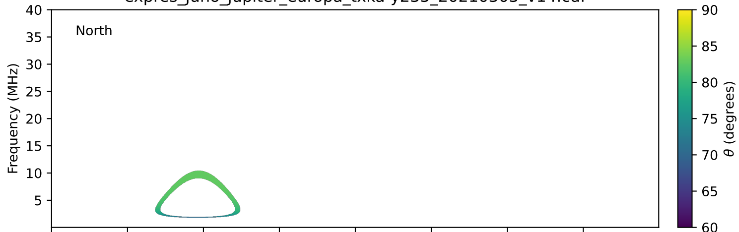
expres_juno_jupiter_europa_txka-y235_20210303_v14.cdf
