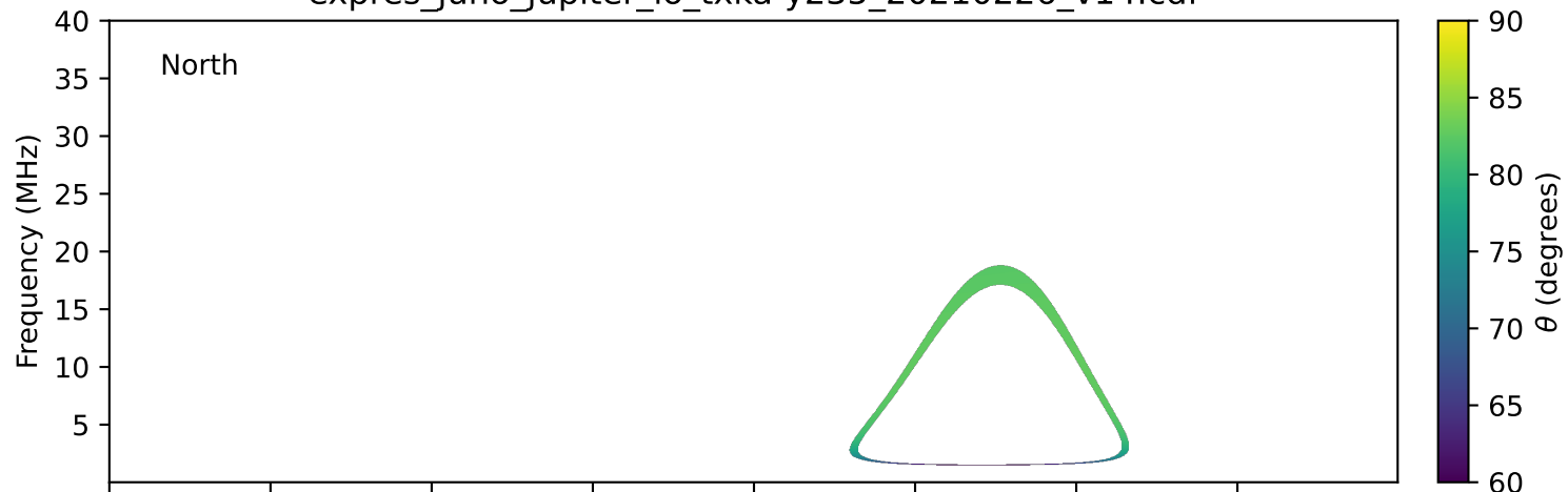
expres_juno_jupiter_io_txka-y235_20210226_v14.cdf
