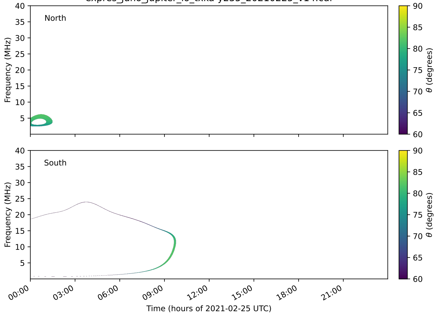
expres_juno_jupiter_io_txka-y235_20210225_v14.cdf
