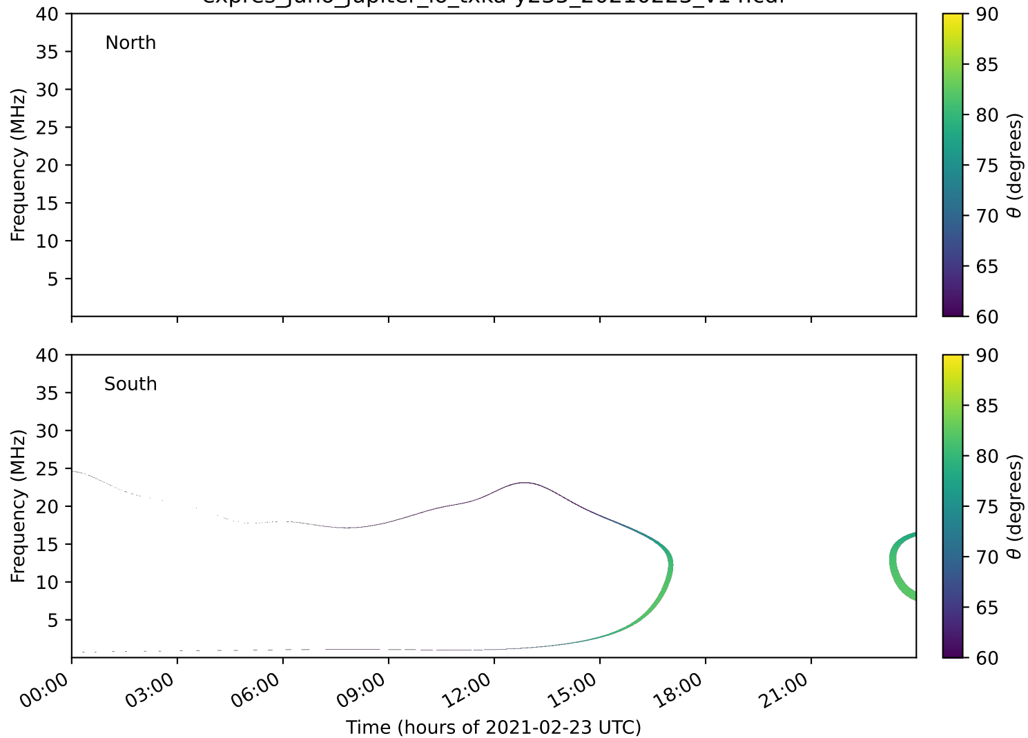
expres_juno_jupiter_io_txka-y235_20210223_v14.cdf
