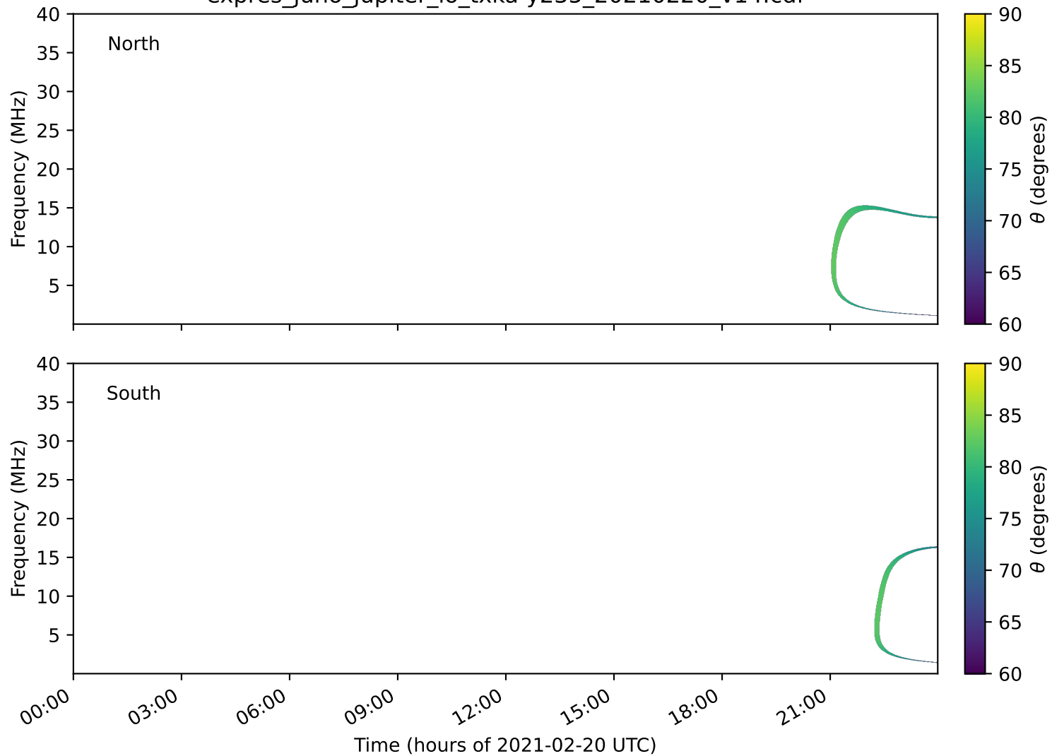
expres_juno_jupiter_io_txka-y235_20210220_v14.cdf
