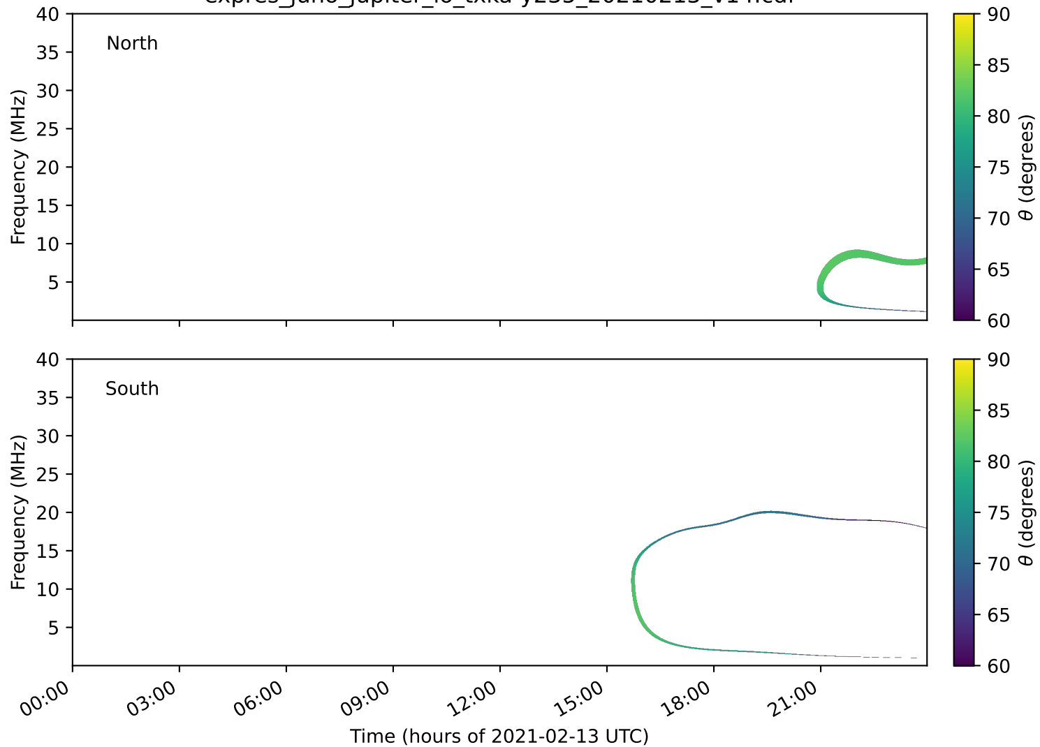
expres_juno_jupiter_io_txka-y235_20210213_v14.cdf
