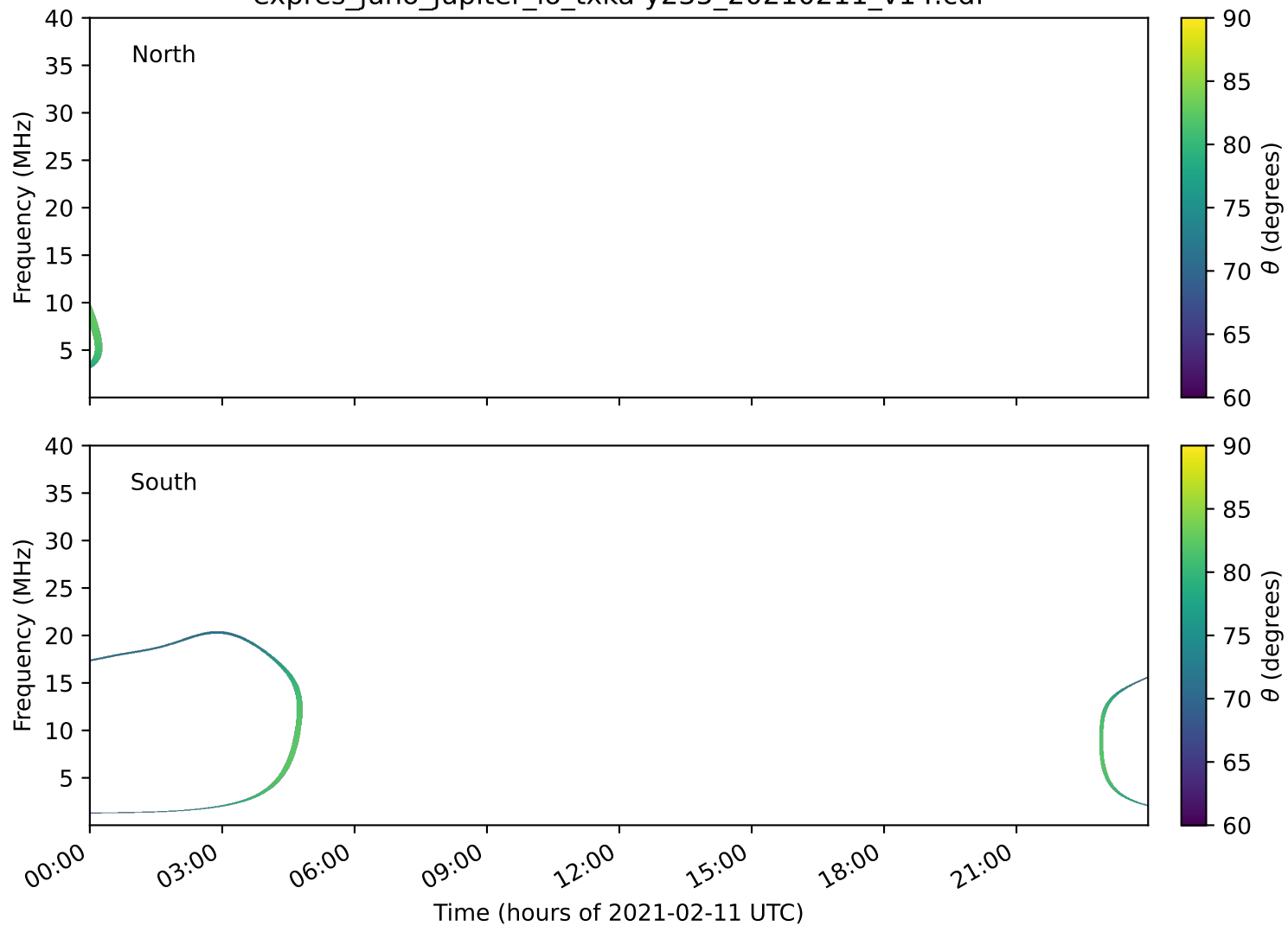
expres_juno_jupiter_io_txka-y235_20210211_v14.cdf
