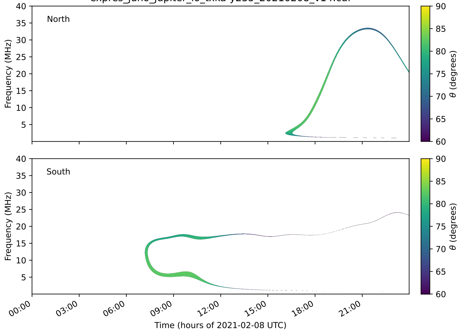
expres_juno_jupiter_io_txka-y235_20210208_v14.cdf
