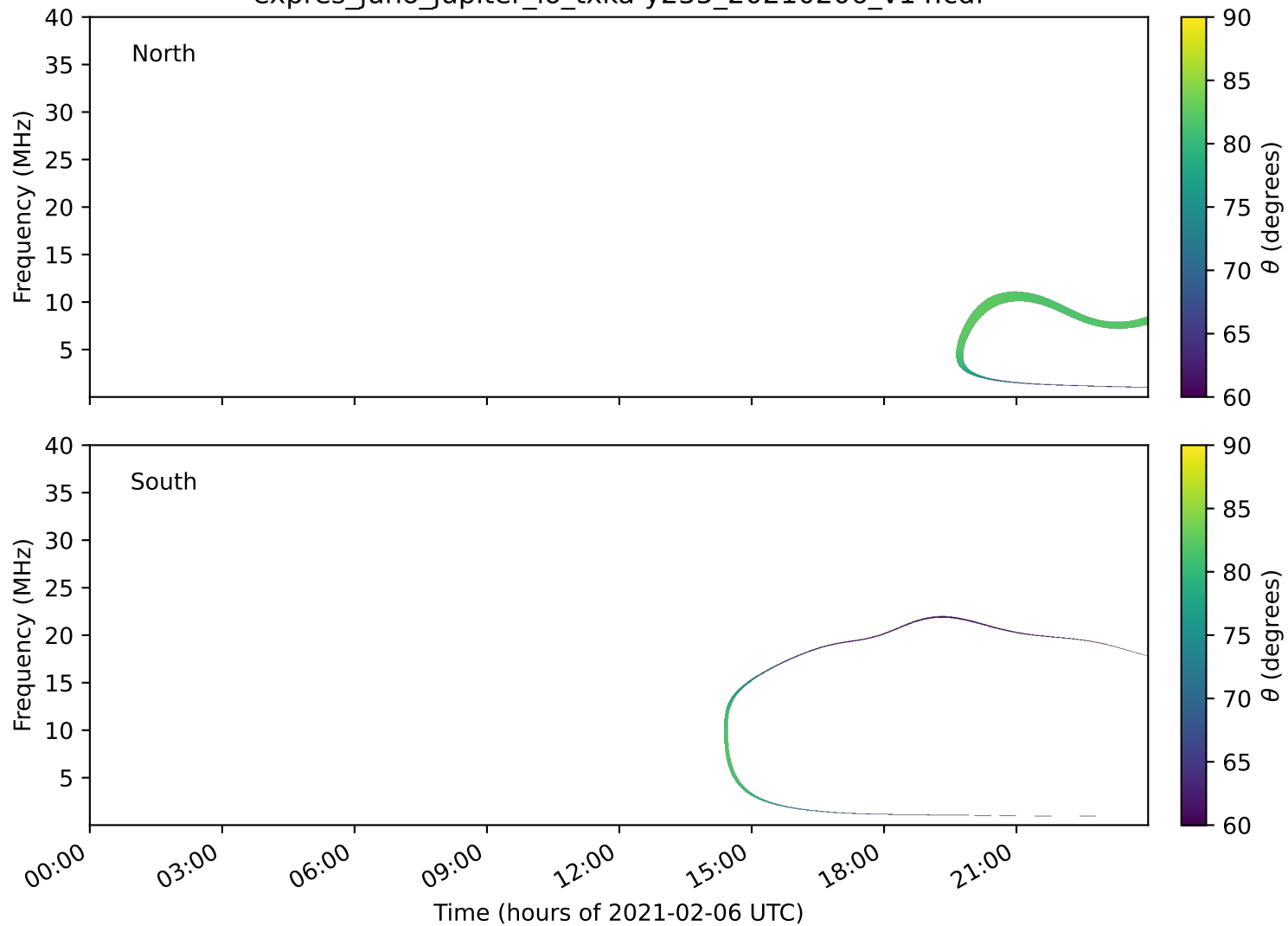
expres_juno_jupiter_io_txka-y235_20210206_v14.cdf
