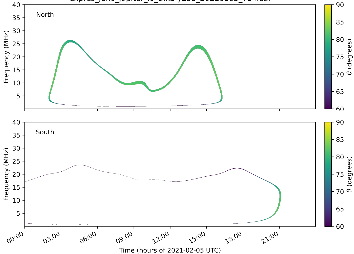
expres_juno_jupiter_io_txka-y235_20210205_v14.cdf
