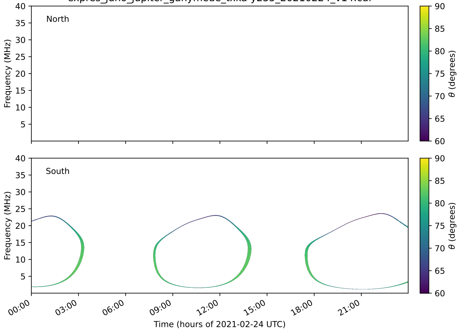
expres_juno_jupiter_ganymede_txka-y235_20210224_v14.cdf
