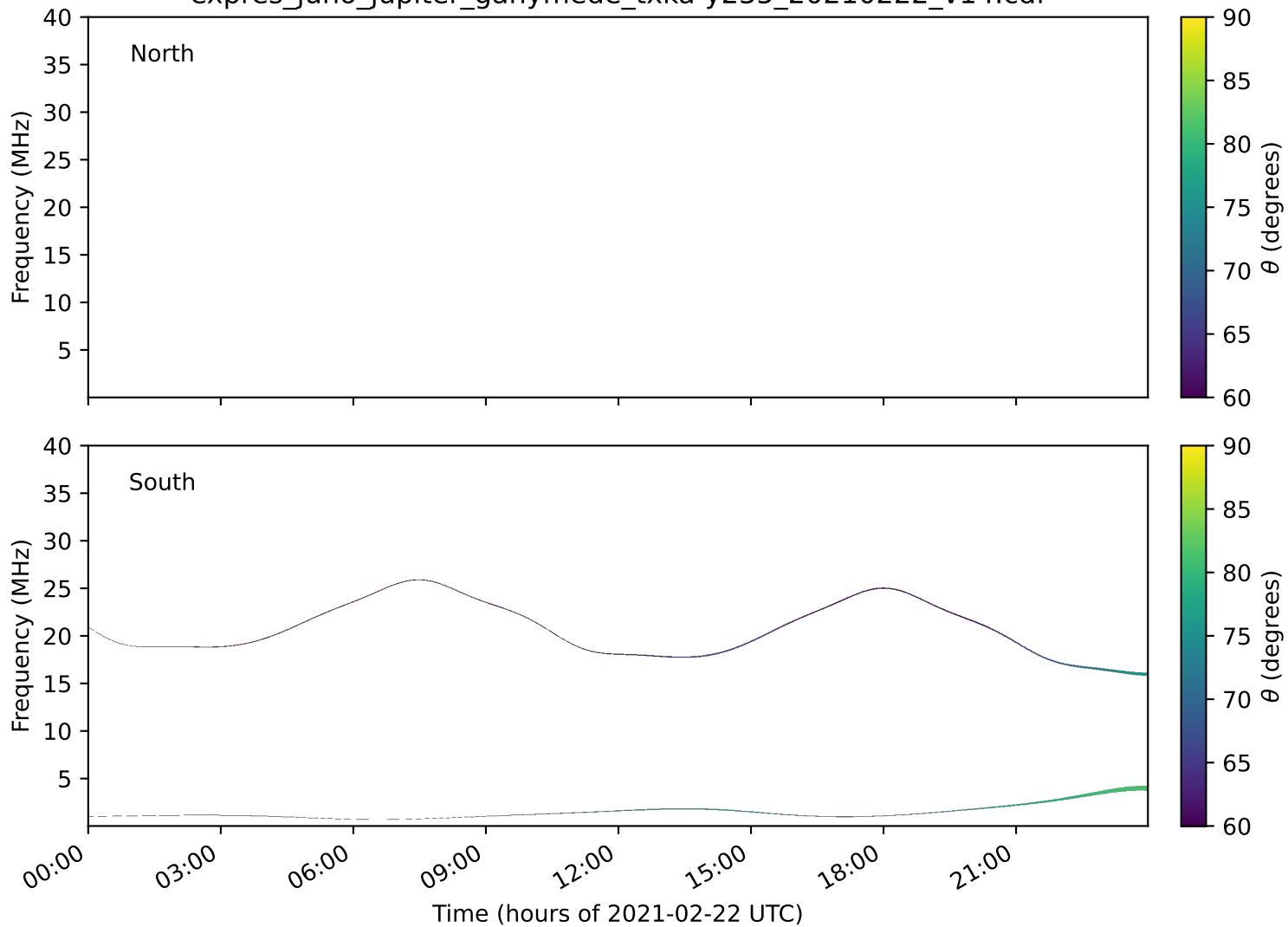
expres_juno_jupiter_ganymede_txka-y235_20210222_v14.cdf
