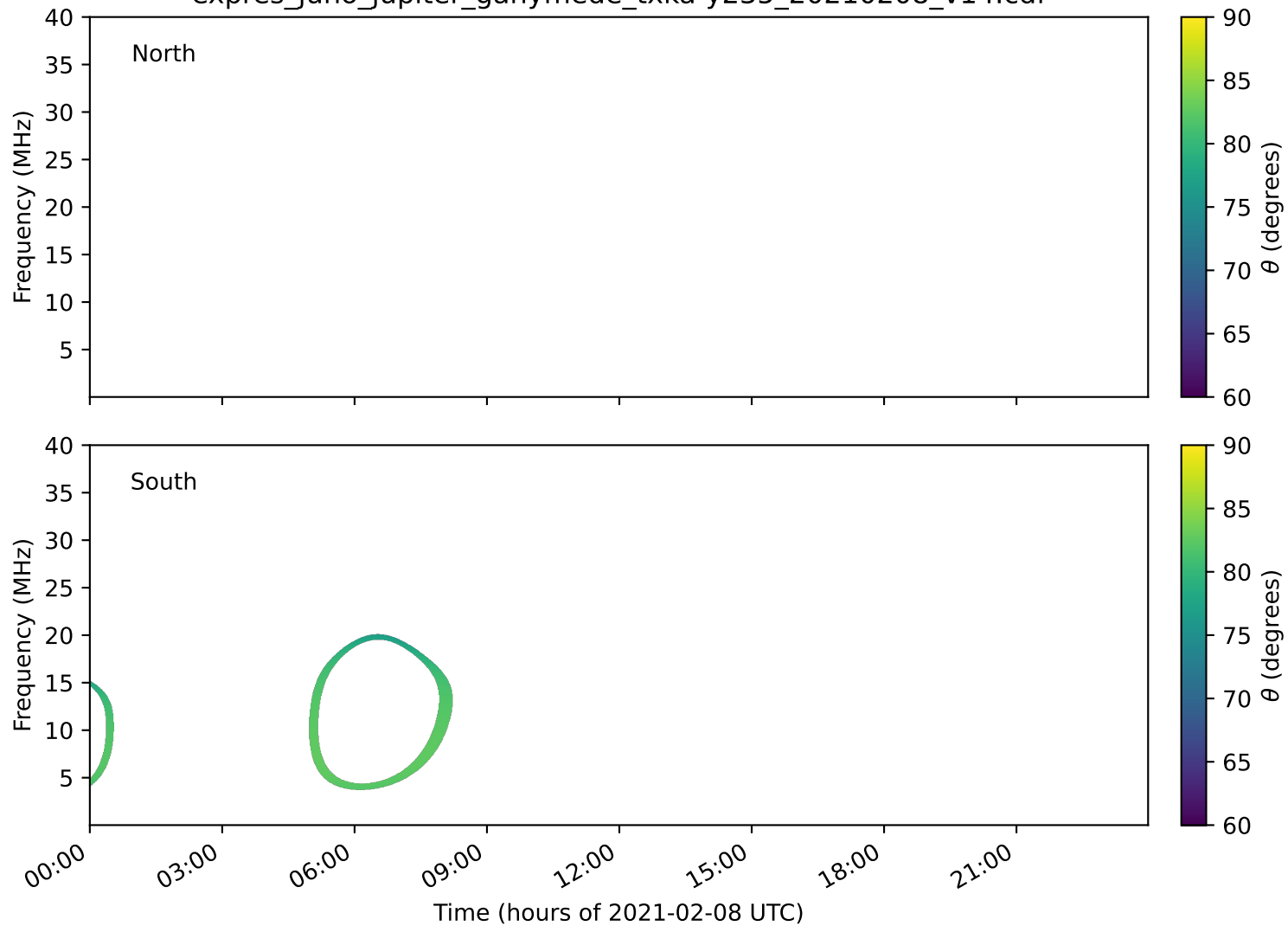
expres_juno_jupiter_ganymede_txka-y235_20210208_v14.cdf
