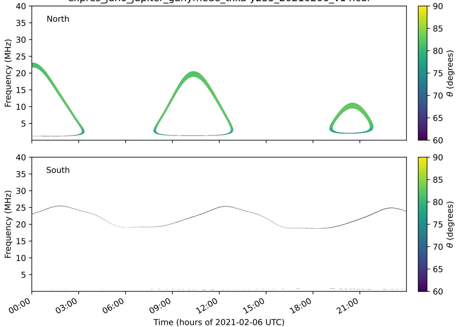
expres_juno_jupiter_ganymede_txka-y235_20210206_v14.cdf
