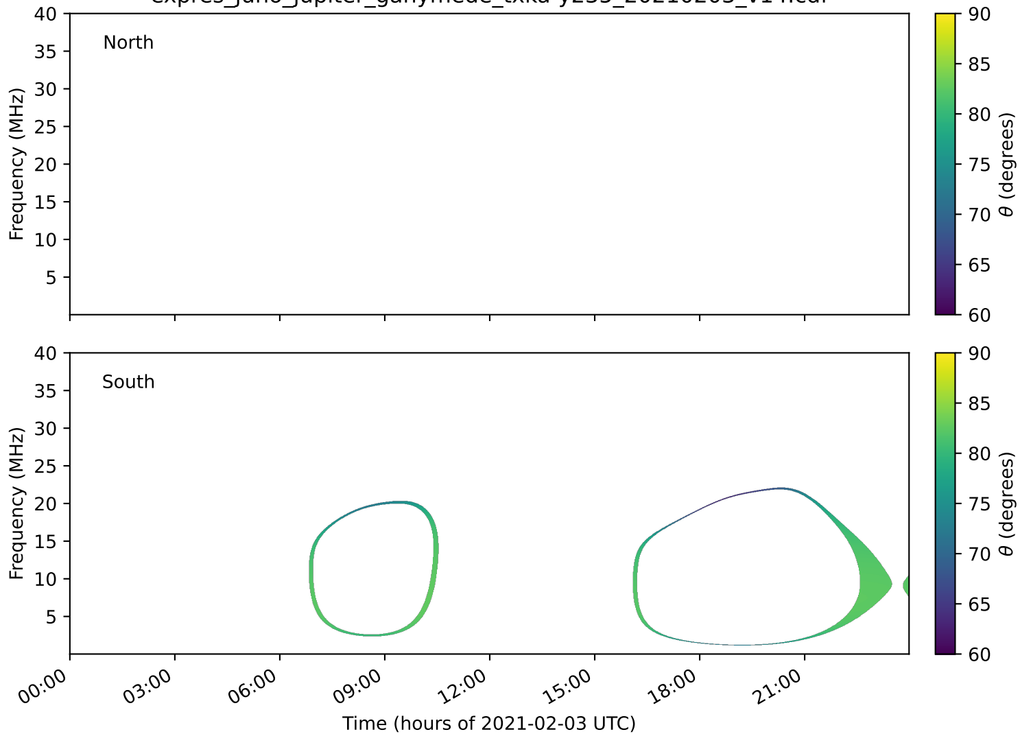
expres_juno_jupiter_ganymede_txka-y235_20210203_v14.cdf
