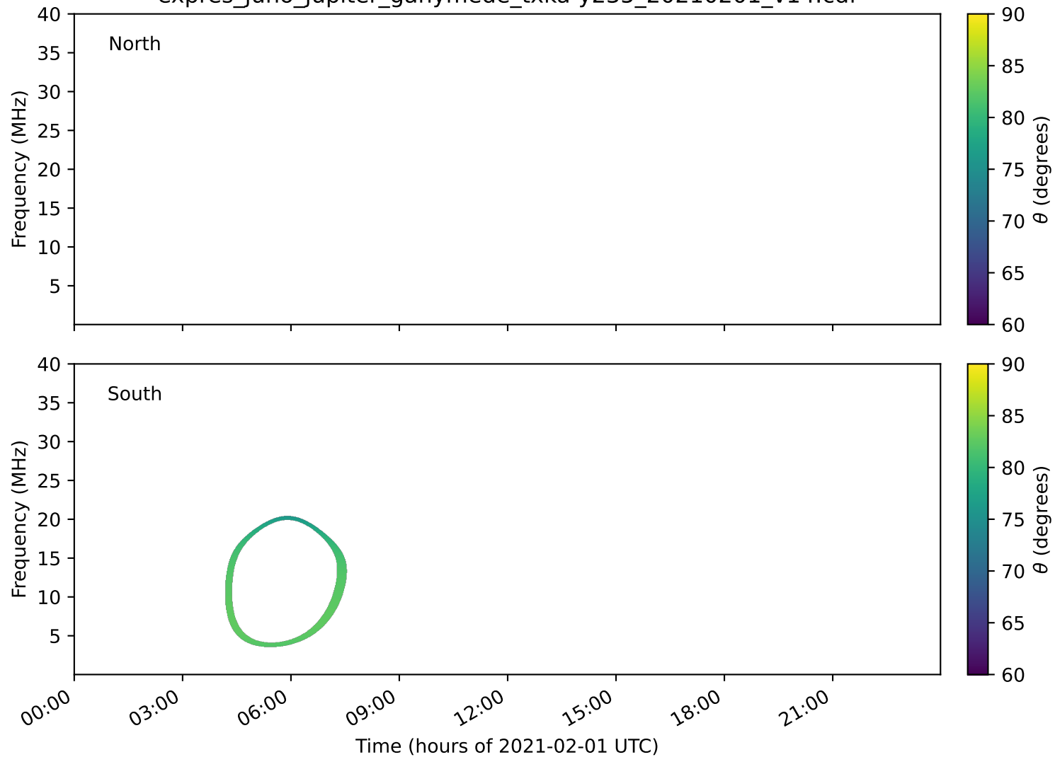
expres_juno_jupiter_ganymede_txka-y235_20210201_v14.cdf
