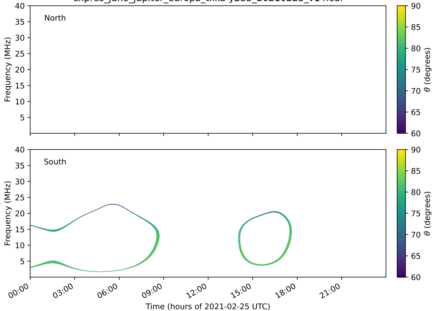
expres_juno_jupiter_europa_txka-y235_20210225_v14.cdf
