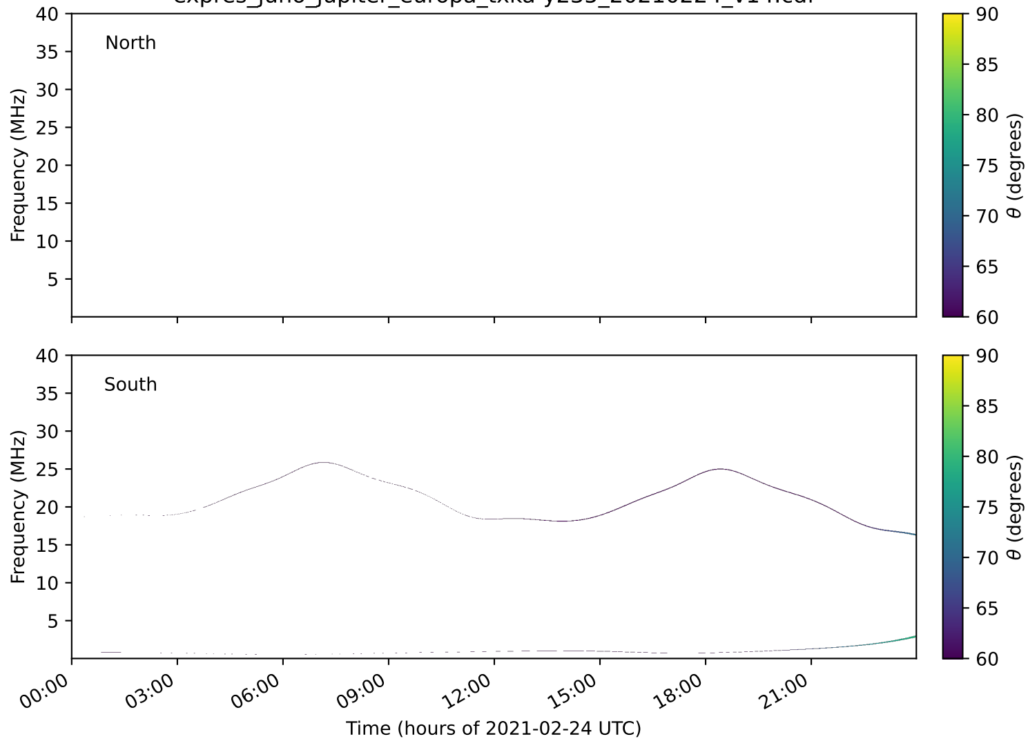
expres_juno_jupiter_europa_txka-y235_20210224_v14.cdf
