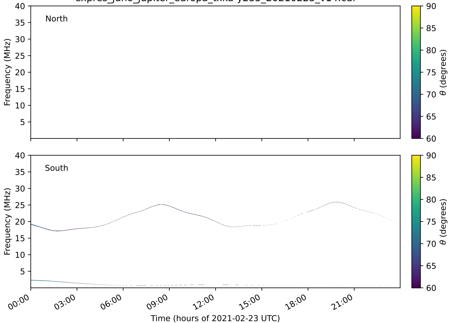
expres_juno_jupiter_europa_txka-y235_20210223_v14.cdf
