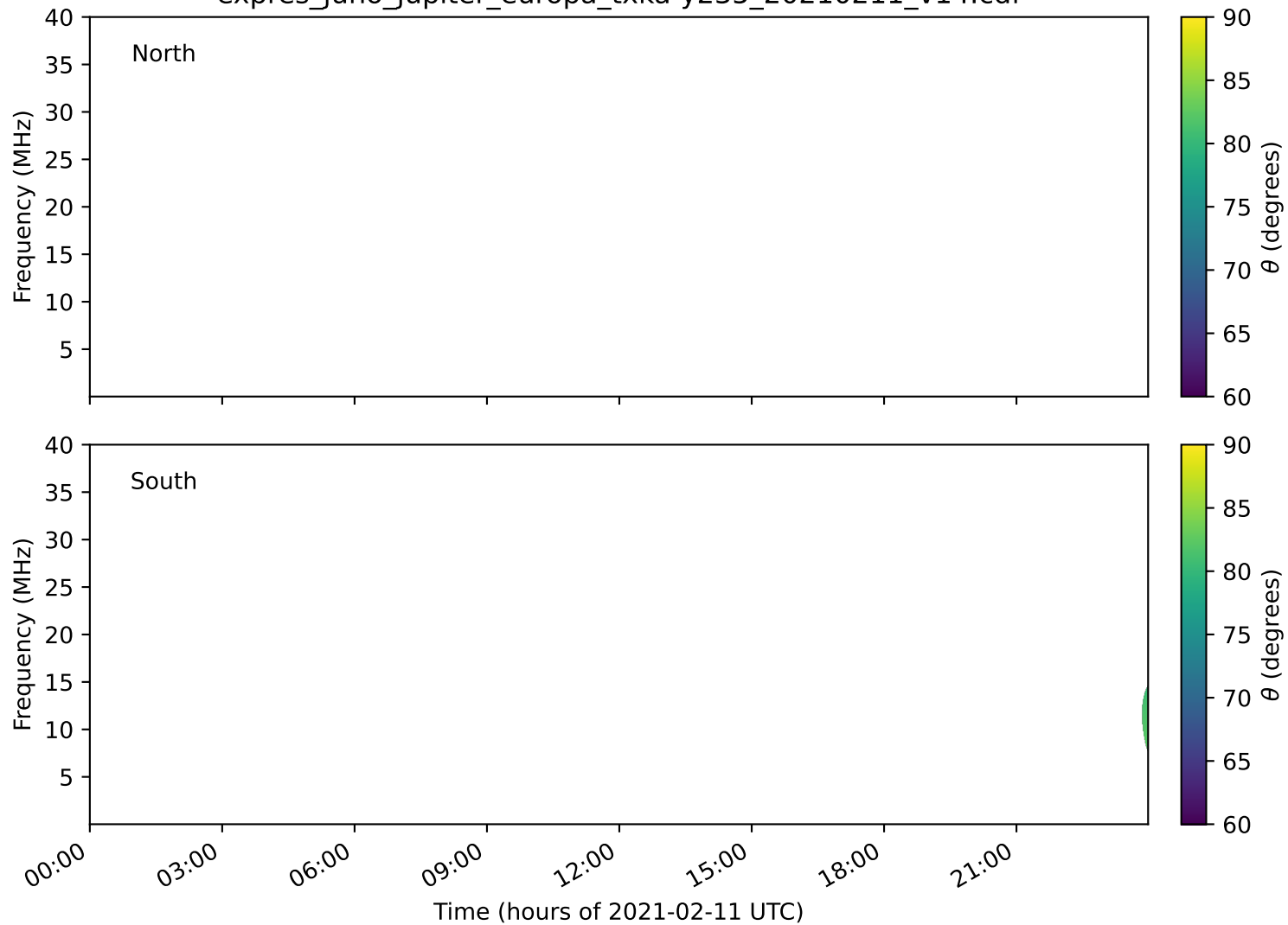
expres_juno_jupiter_europa_txka-y235_20210211_v14.cdf
