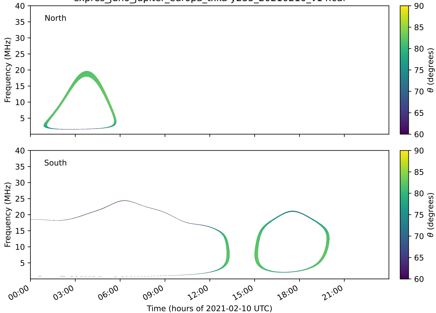
expres_juno_jupiter_europa_txka-y235_20210210_v14.cdf
