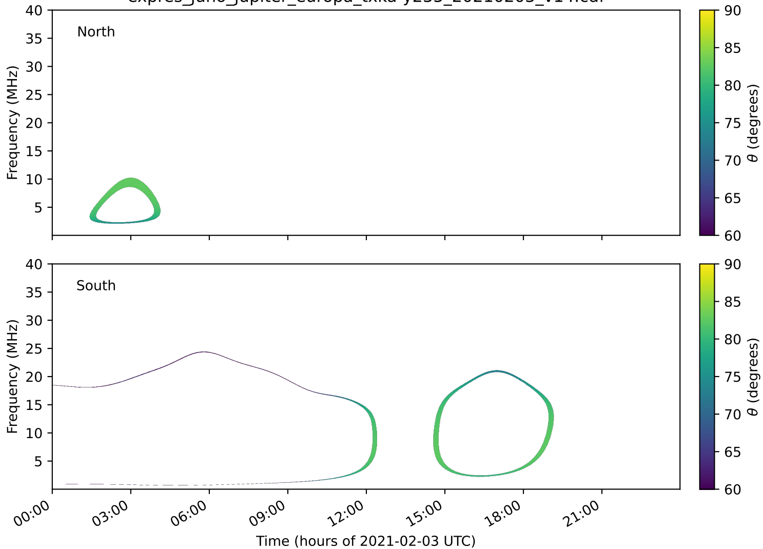
expres_juno_jupiter_europa_txka-y235_20210203_v14.cdf
