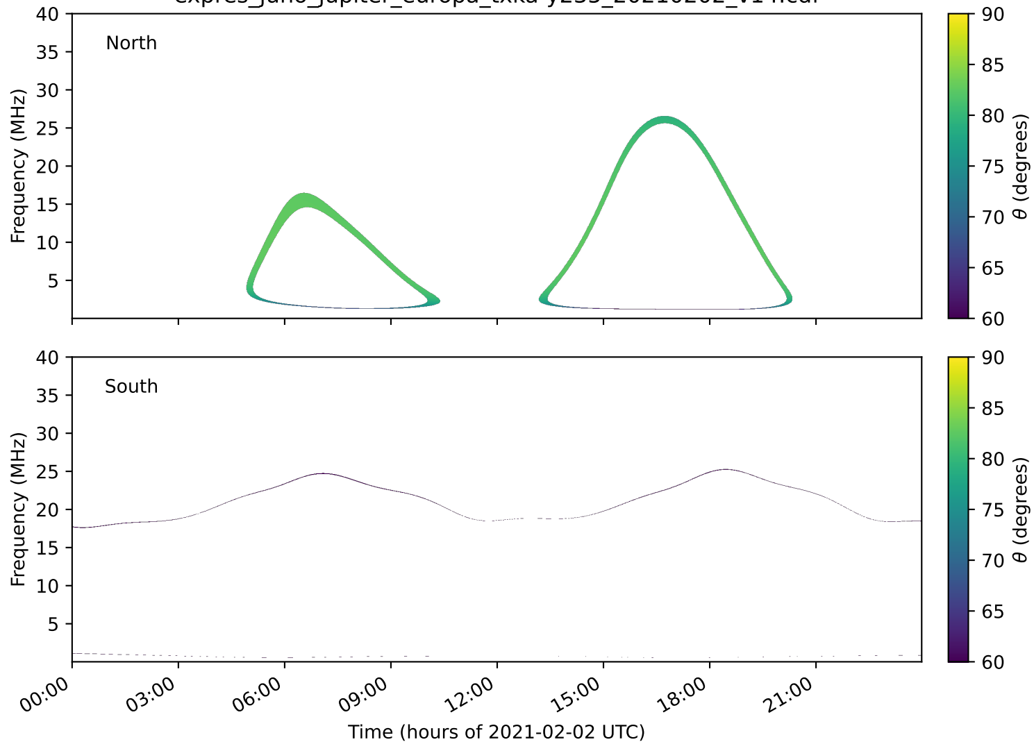
expres_juno_jupiter_europa_txka-y235_20210202_v14.cdf
