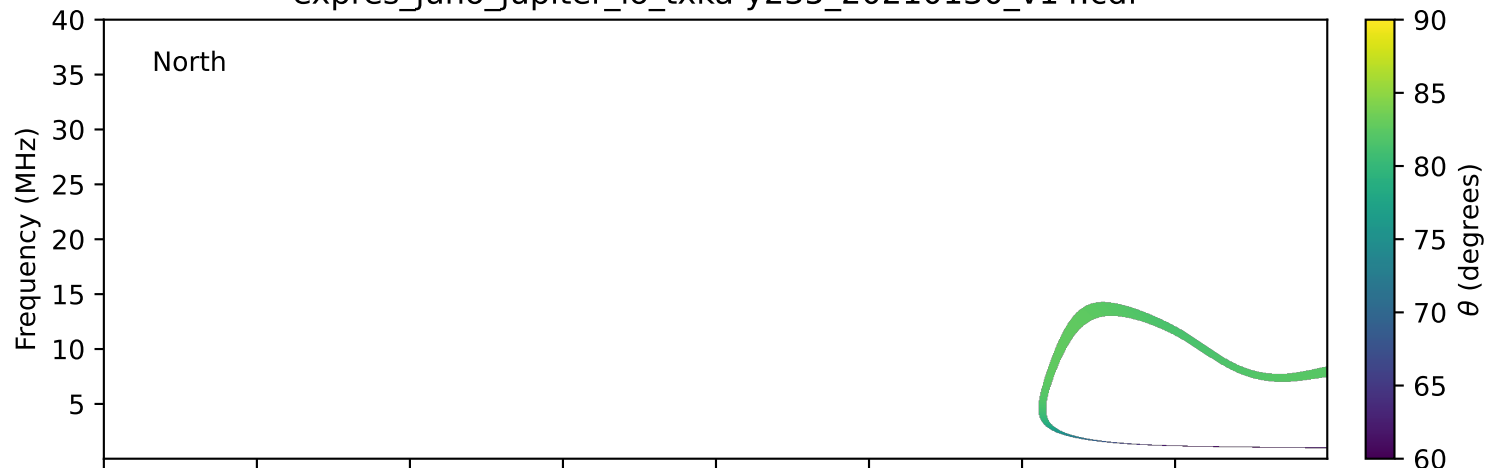
expres_juno_jupiter_io_txka-y235_20210130_v14.cdf
