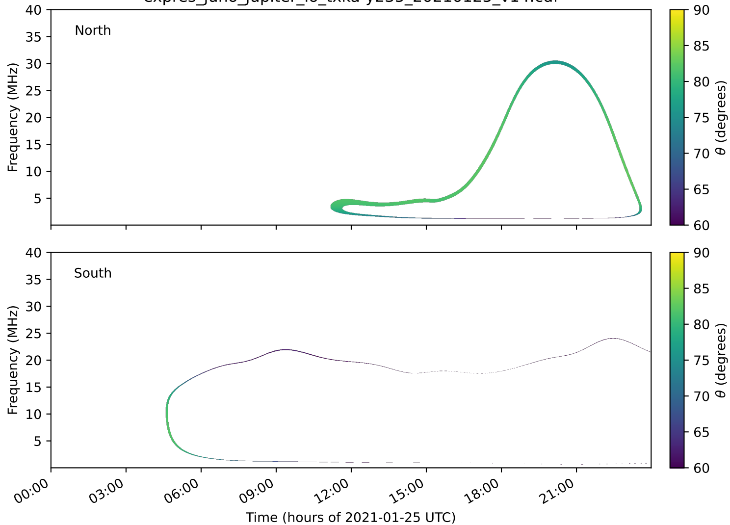
expres_juno_jupiter_io_txka-y235_20210125_v14.cdf
