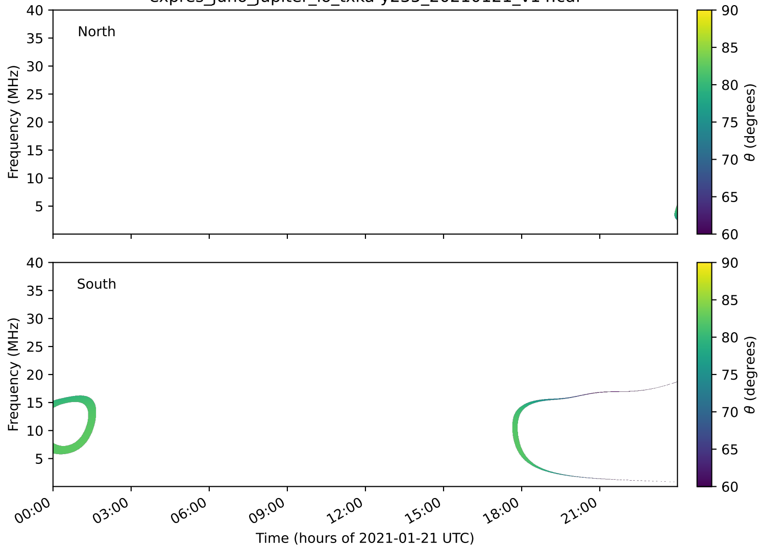
expres_juno_jupiter_io_txka-y235_20210121_v14.cdf
