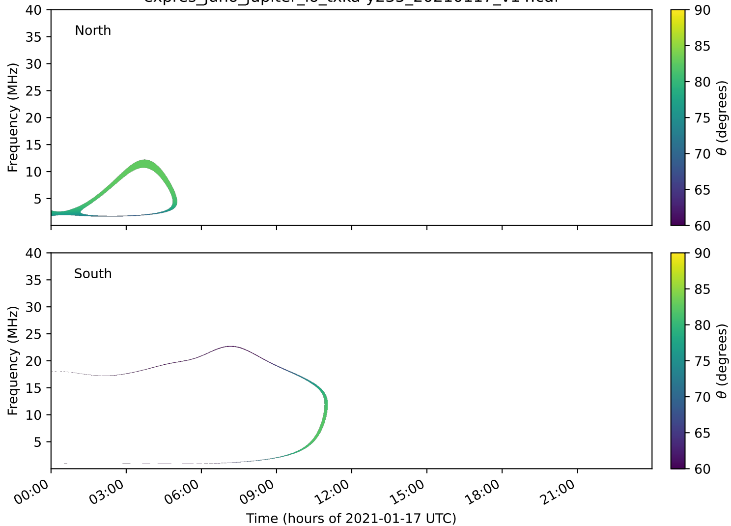
expres_juno_jupiter_io_txka-y235_20210117_v14.cdf
