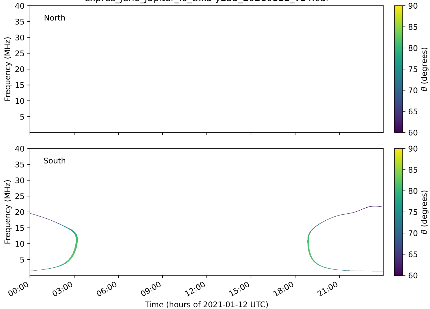
expres_juno_jupiter_io_txka-y235_20210112_v14.cdf
