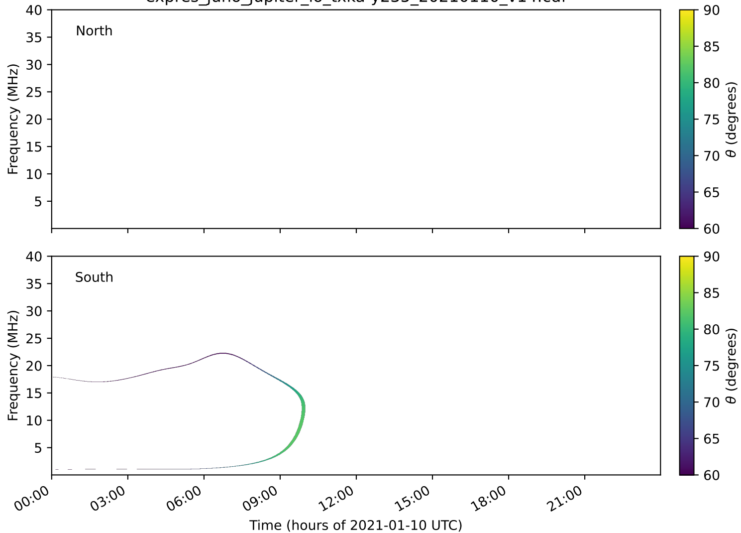
expres_juno_jupiter_io_txka-y235_20210110_v14.cdf
