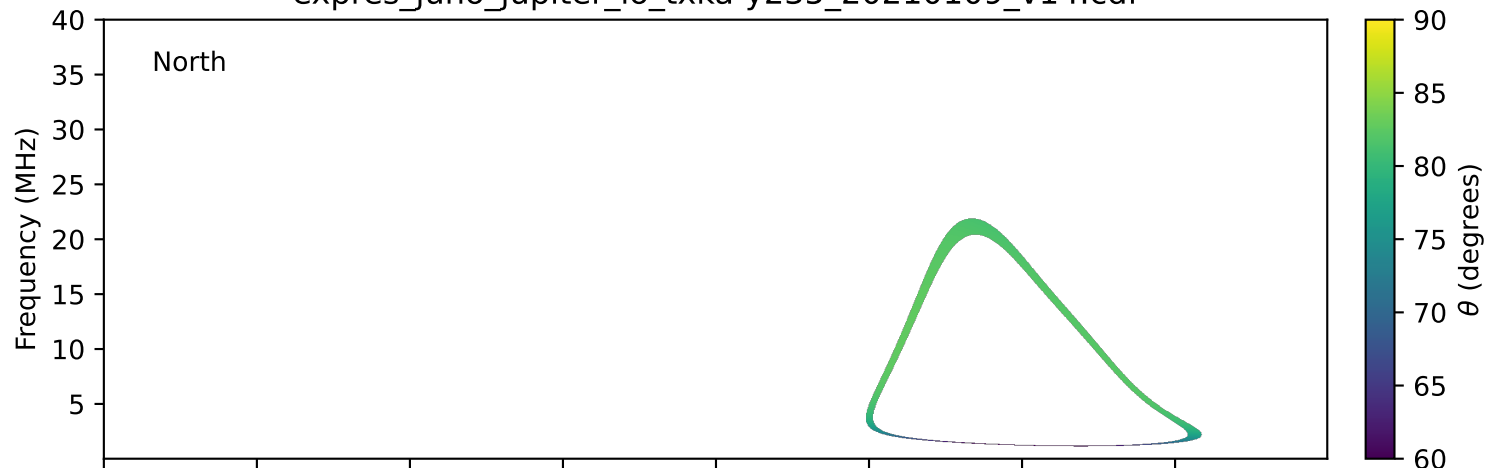
expres_juno_jupiter_io_txka-y235_20210109_v14.cdf
