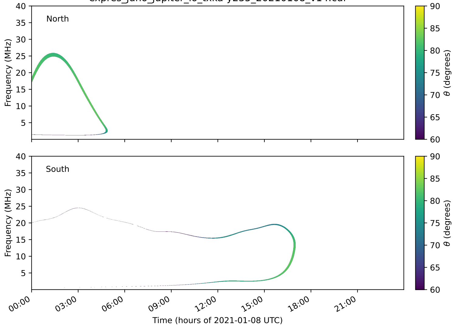
expres_juno_jupiter_io_txka-y235_20210108_v14.cdf
