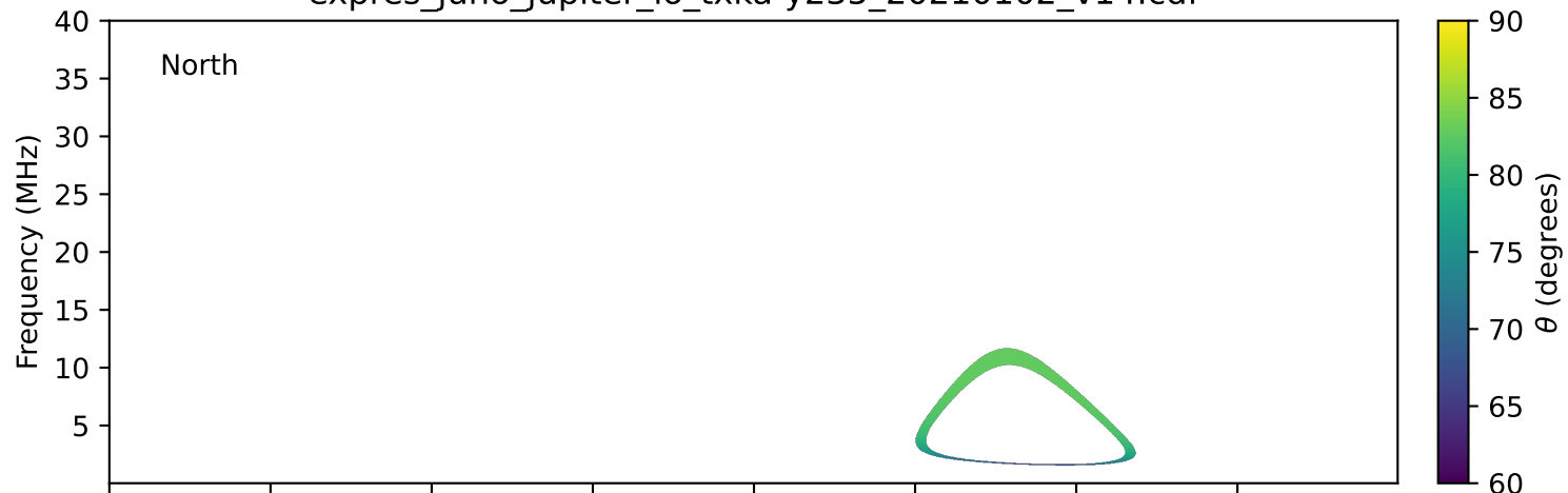
expres_juno_jupiter_io_txka-y235_20210102_v14.cdf
