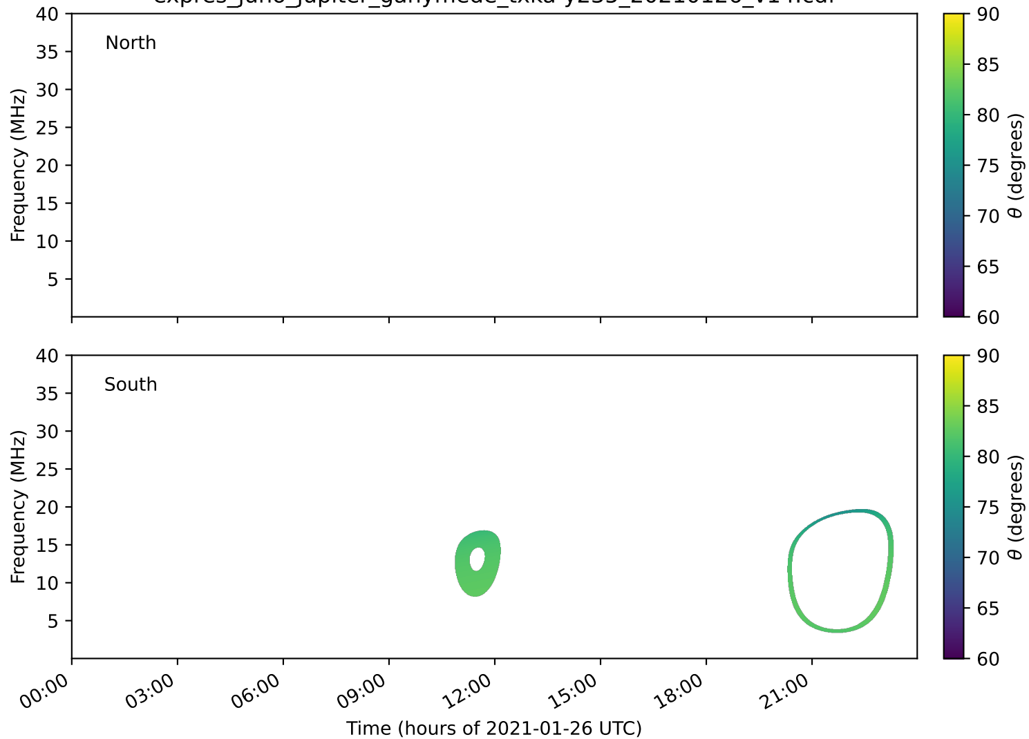
expres_juno_jupiter_ganymede_txka-y235_20210126_v14.cdf
