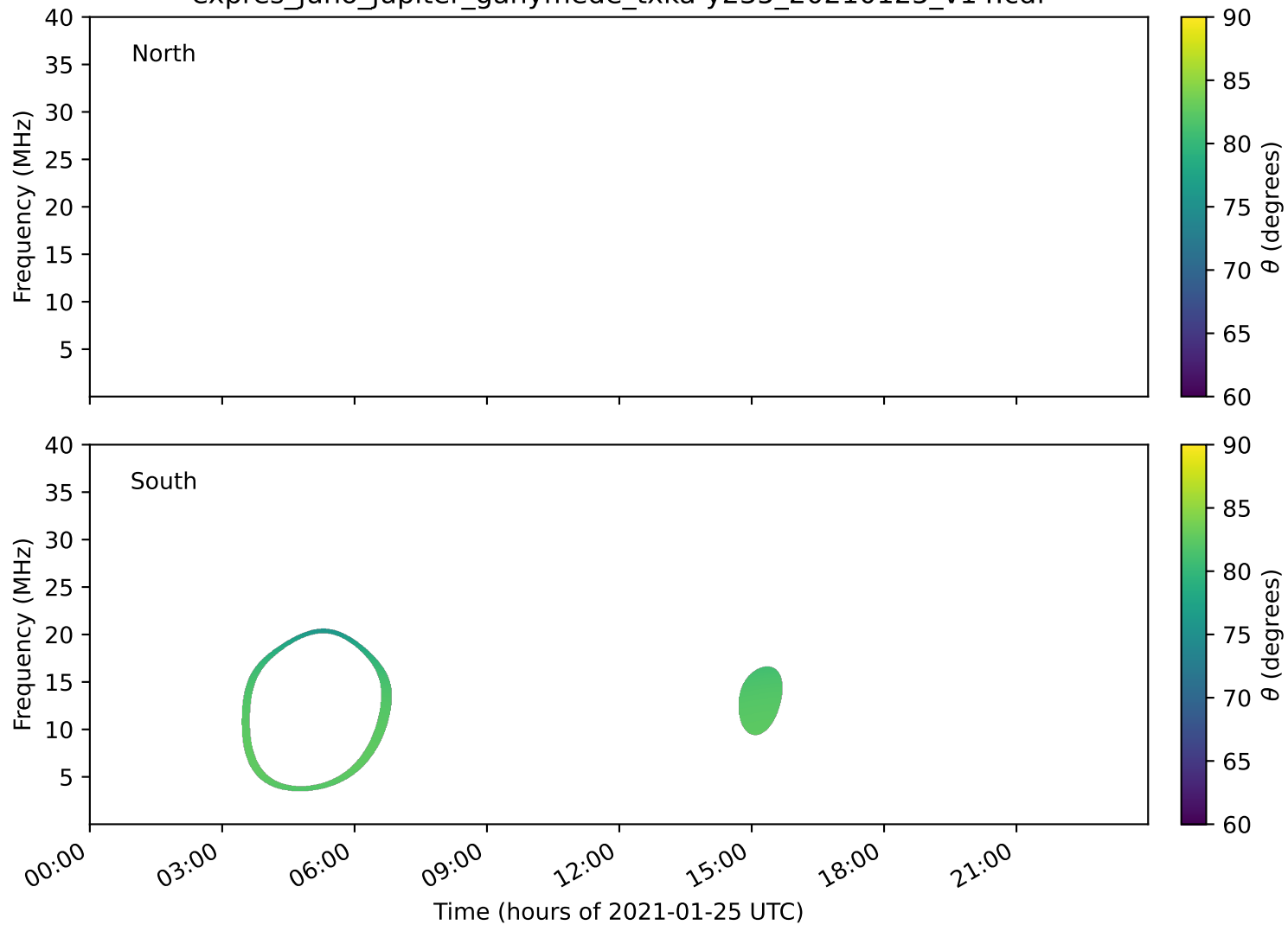
expres_juno_jupiter_ganymede_txka-y235_20210125_v14.cdf
