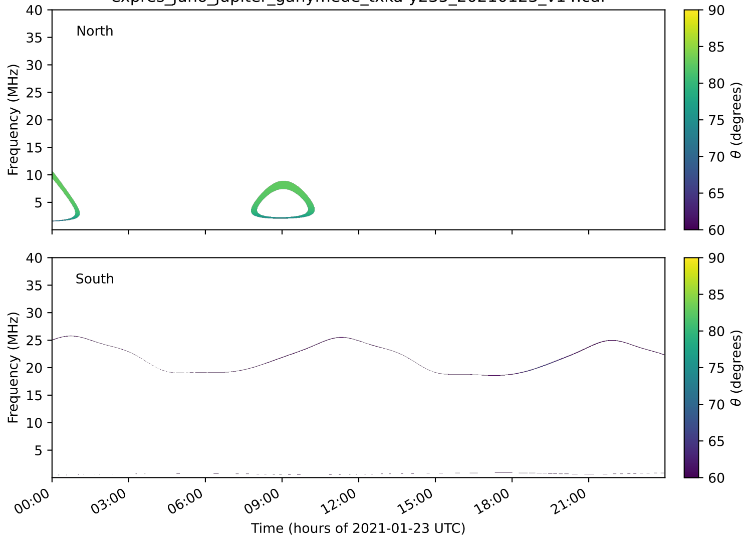
expres_juno_jupiter_ganymede_txka-y235_20210123_v14.cdf
