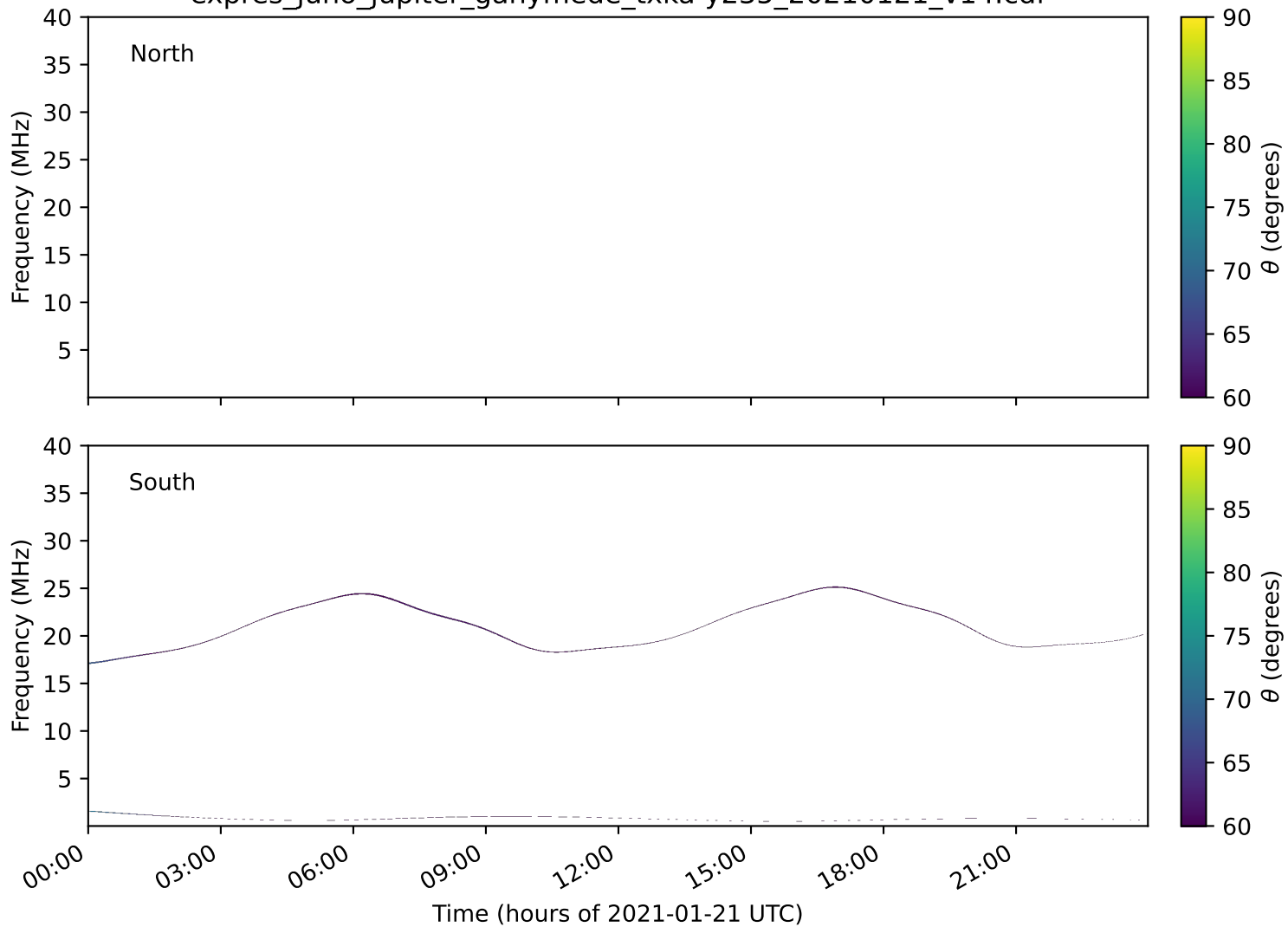
expres_juno_jupiter_ganymede_txka-y235_20210121_v14.cdf
