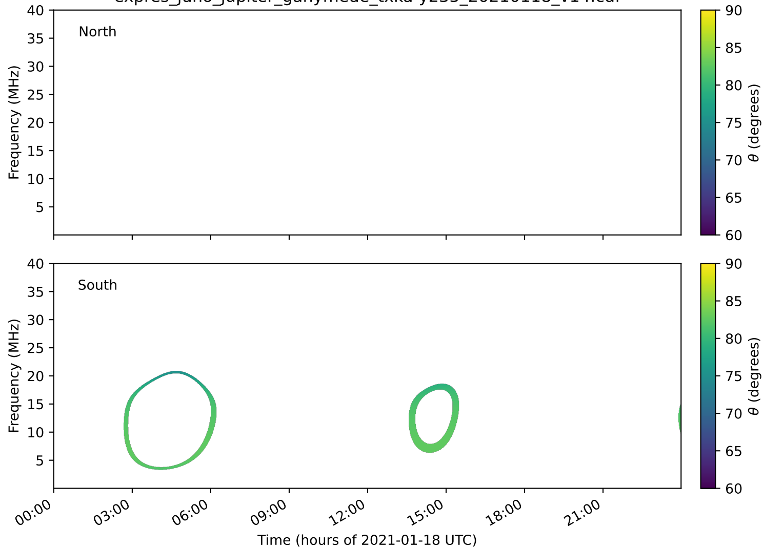
expres_juno_jupiter_ganymede_txka-y235_20210118_v14.cdf
