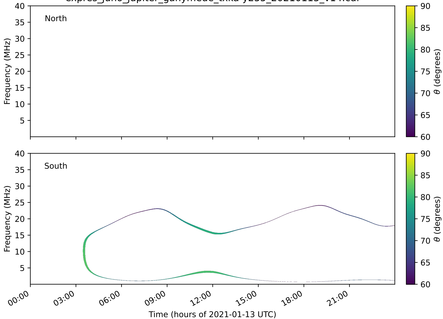
expres_juno_jupiter_ganymede_txka-y235_20210113_v14.cdf
