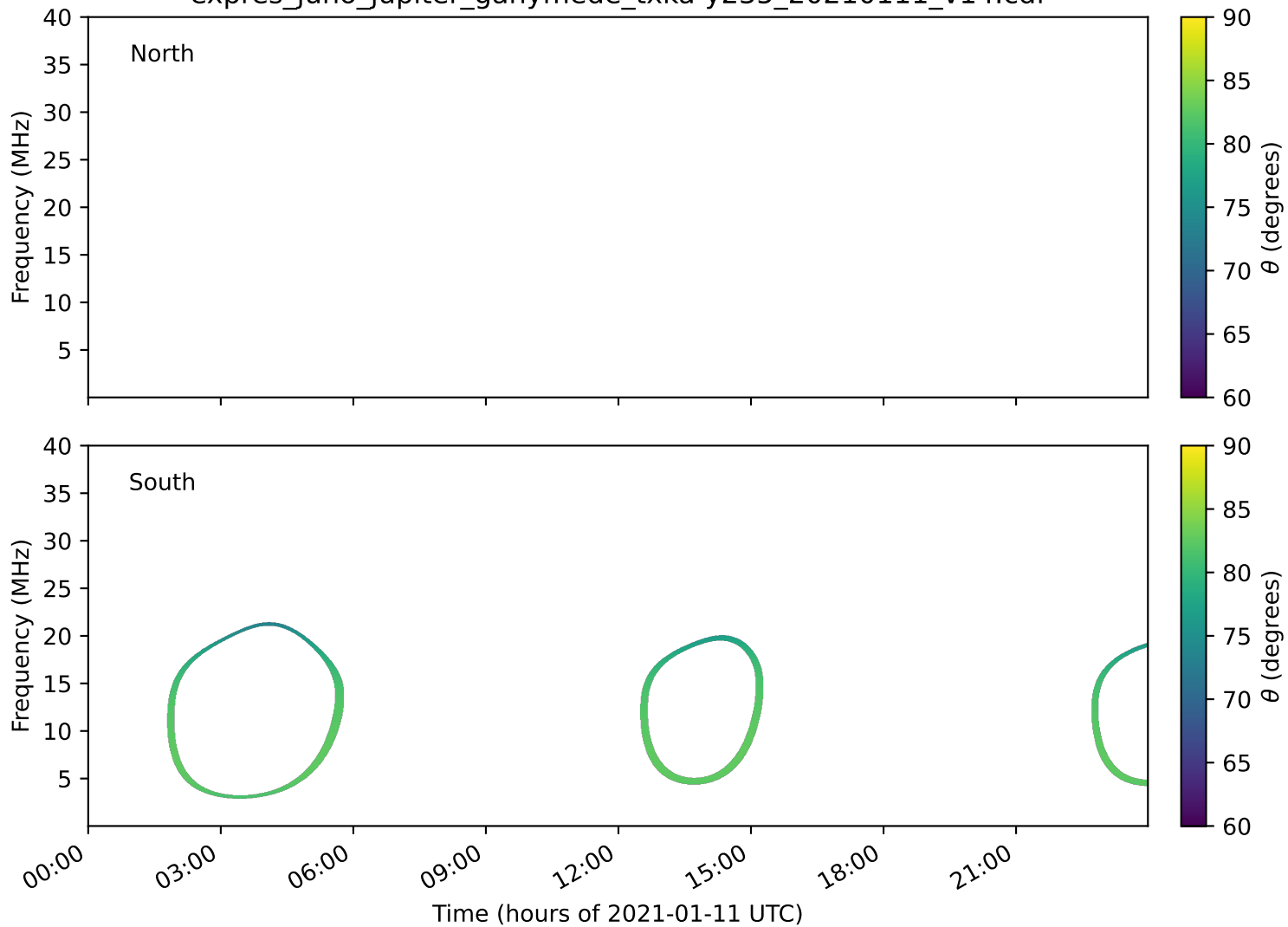
expres_juno_jupiter_ganymede_txka-y235_20210111_v14.cdf
