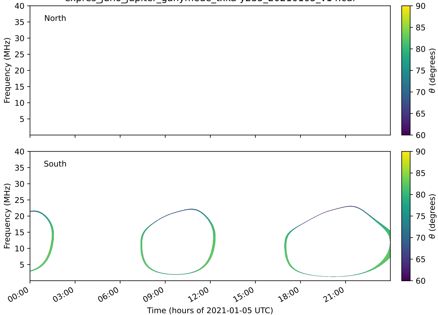
expres_juno_jupiter_ganymede_txka-y235_20210105_v14.cdf
