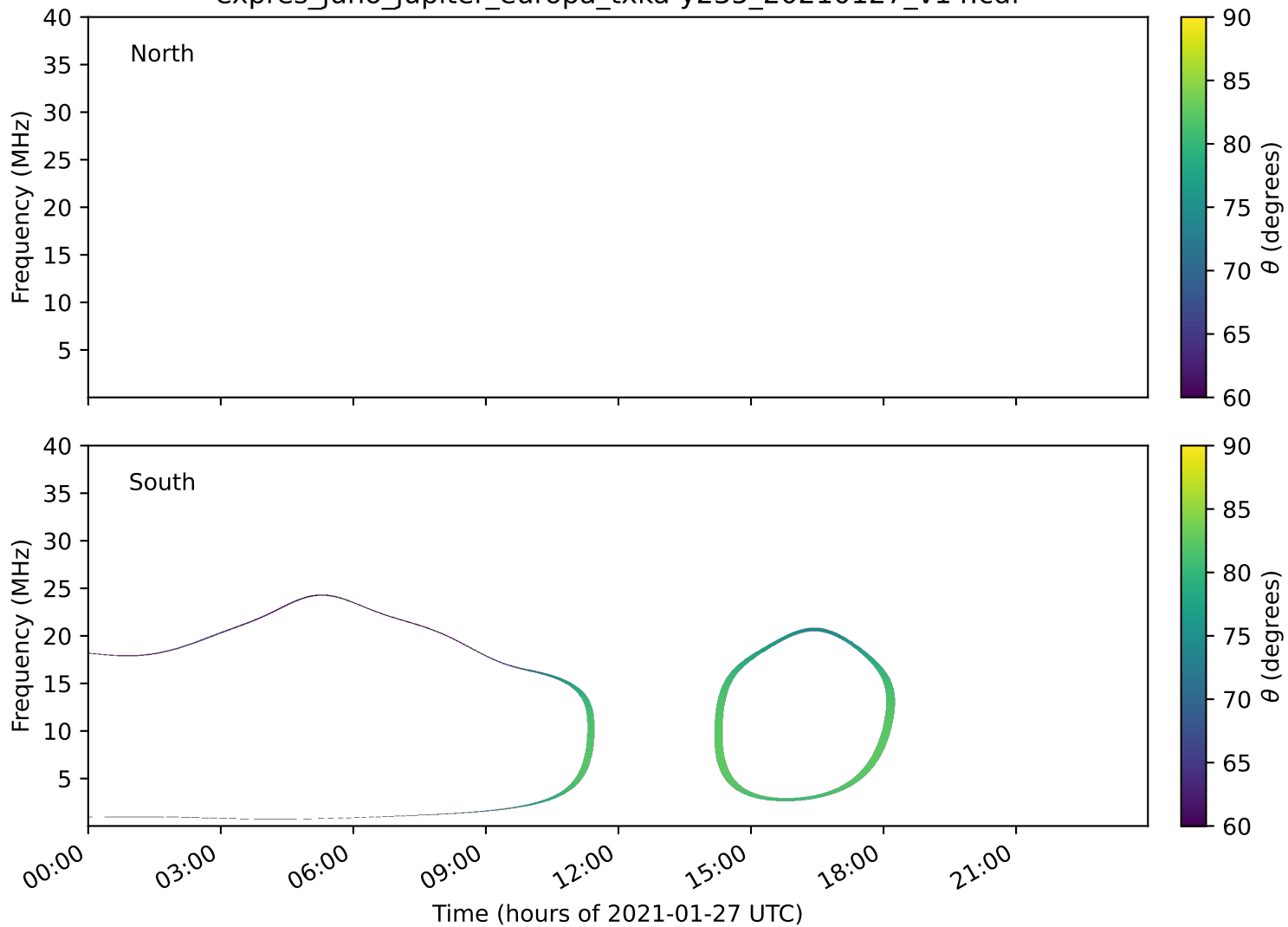
expres_juno_jupiter_europa_txka-y235_20210127_v14.cdf
