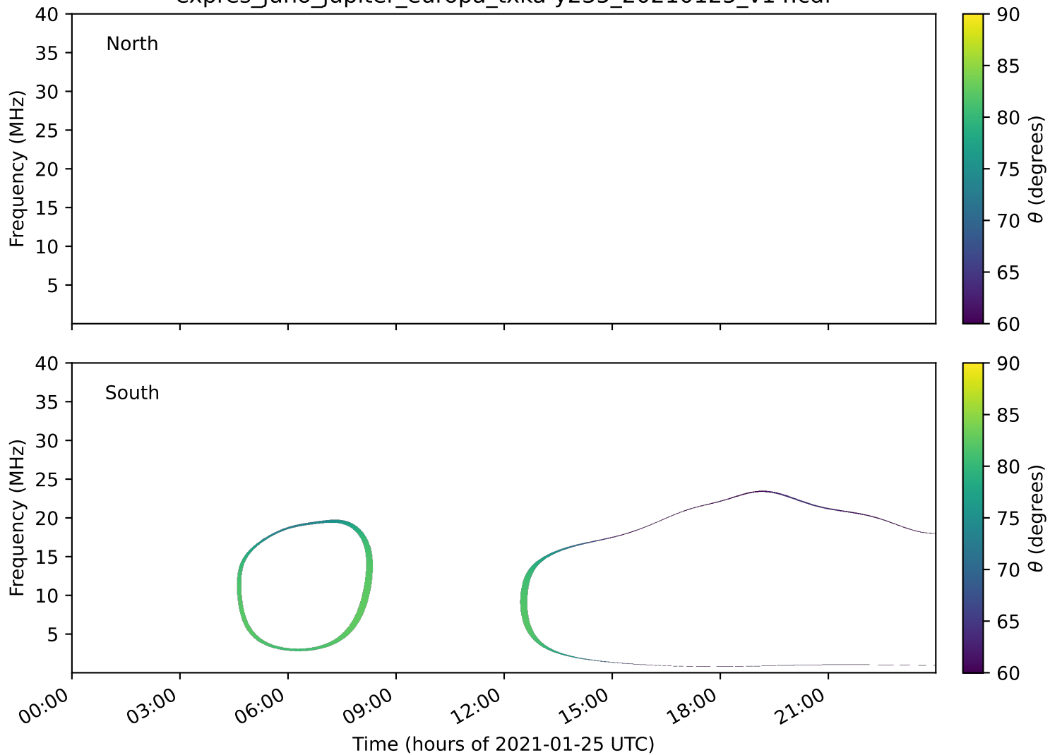
expres_juno_jupiter_europa_txka-y235_20210125_v14.cdf
