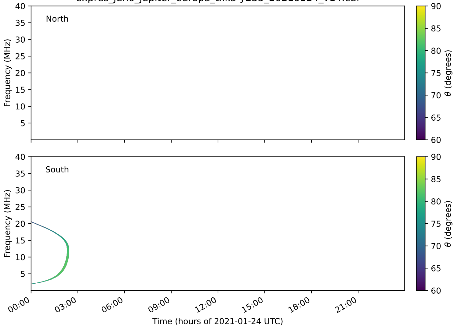
expres_juno_jupiter_europa_txka-y235_20210124_v14.cdf
