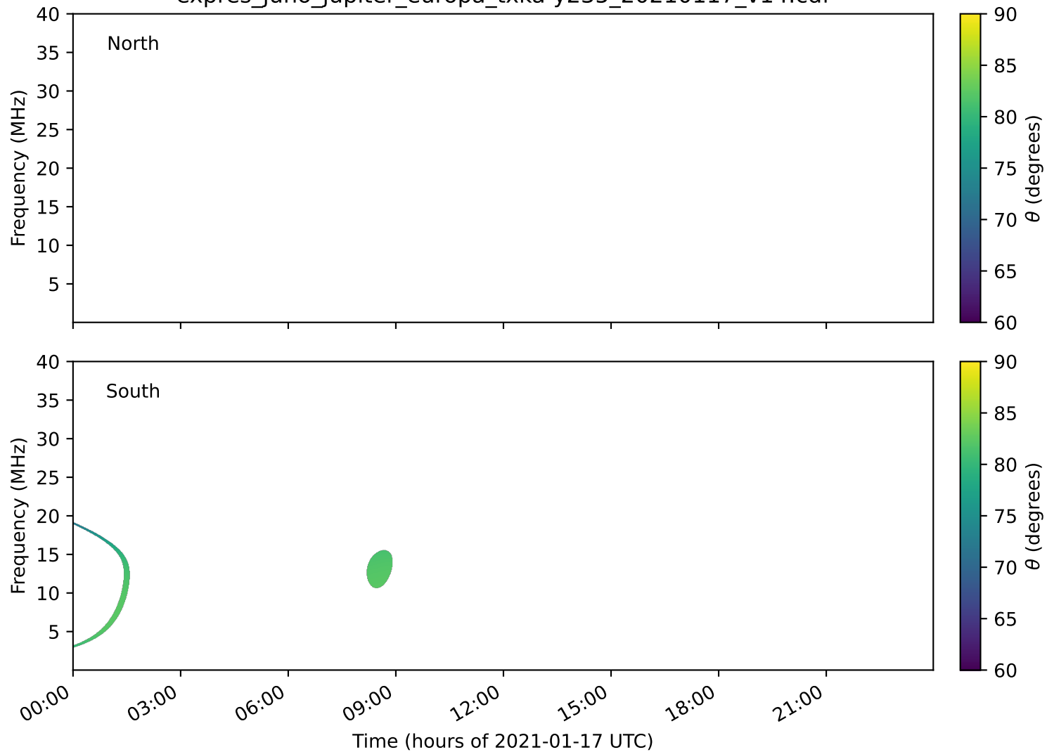
expres_juno_jupiter_europa_txka-y235_20210117_v14.cdf
